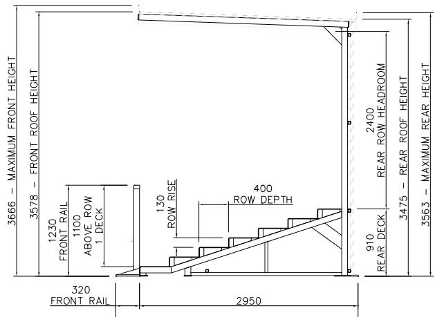
Cut-away to seating
