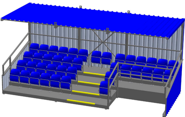
50 seat module with rails, half cladding and left hand wheelchair cutout
