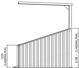
With side rail and half cladding
