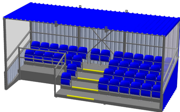
50 seat module with rails, half cladding, perspex window and right hand wheelchair cutout.
