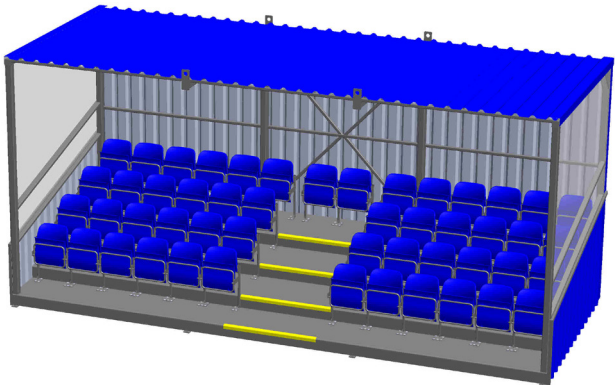
50 seat module with rails, half cladding and perspex window
