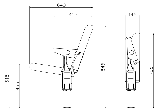
Standard back model, tread fixed
