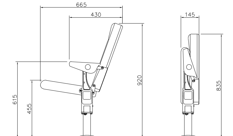
High back model, tread fixed
