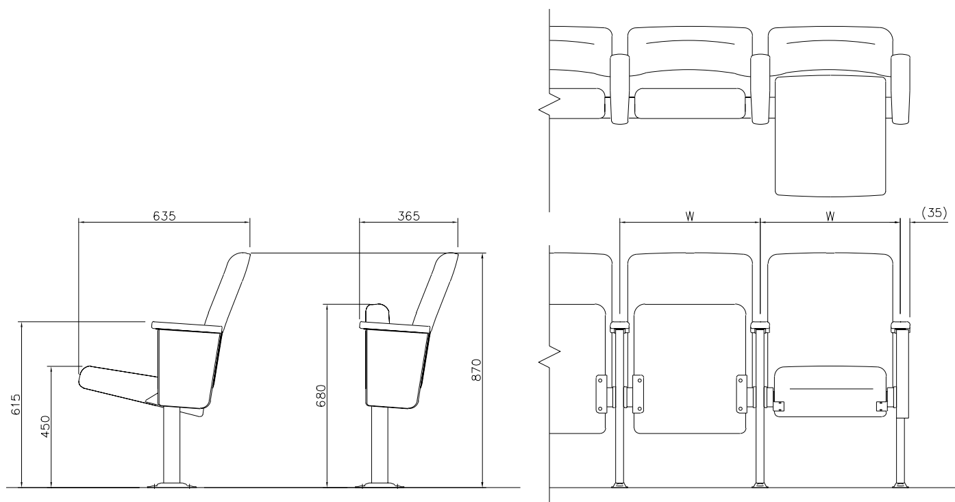
Drawing shows tread fixed chair. Height measurements and taken at seat centre. All dimensions are nominal.
