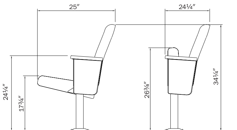
Drawing shows tread fixed chair. Height measurements and taken at seat center. All dimensions are nominal.
