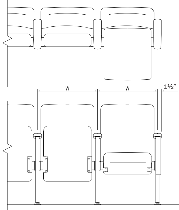
Drawing shows tread fixed chair. Height measurements and taken at seat center. All dimensions are nominal.
